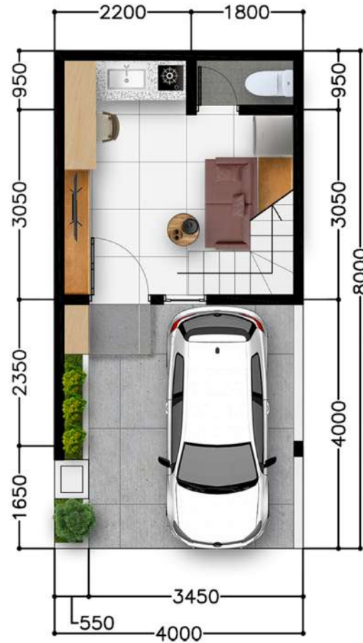
denah lantai 1
