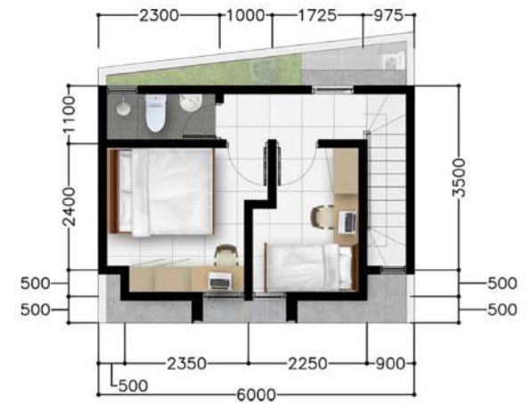
denah lantai 2
