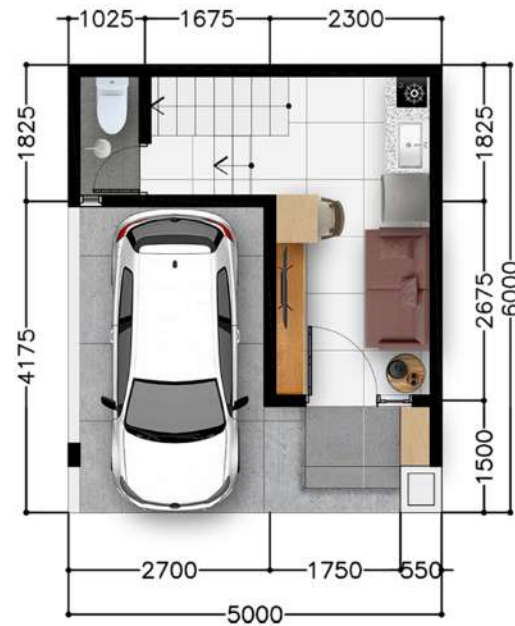
denah lantai 1
