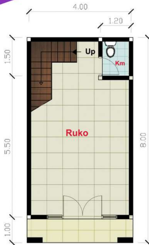
DENAH LT.DASAR
