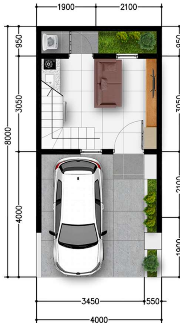
denah lantai 1
