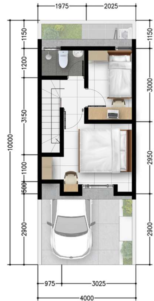
denah lantai 2
