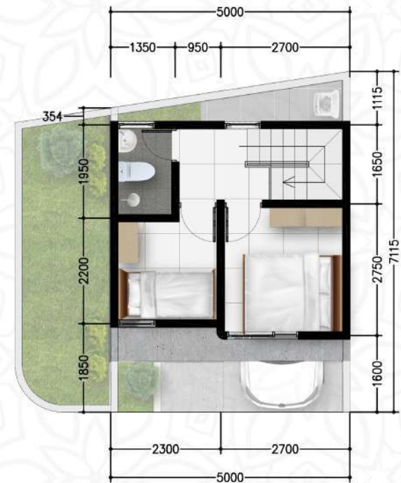
denah lantai 2
