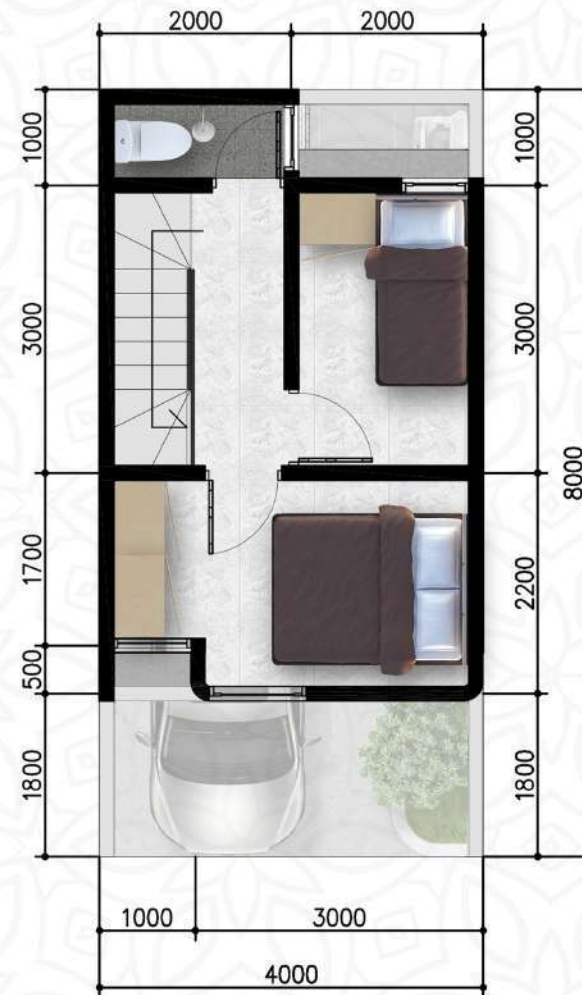
denah lantai 2
