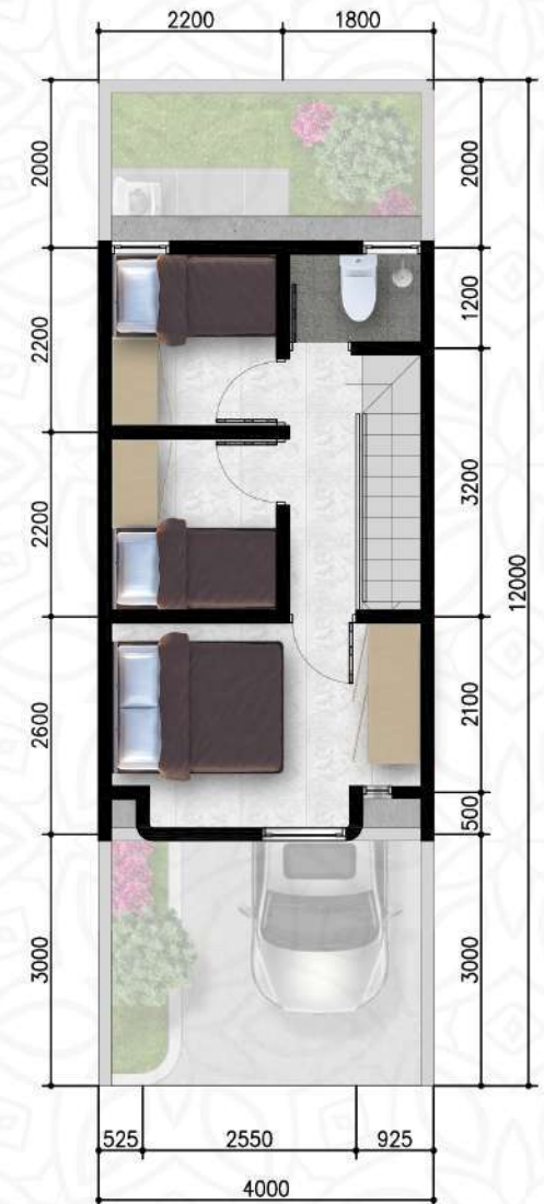
denah lantai 2
